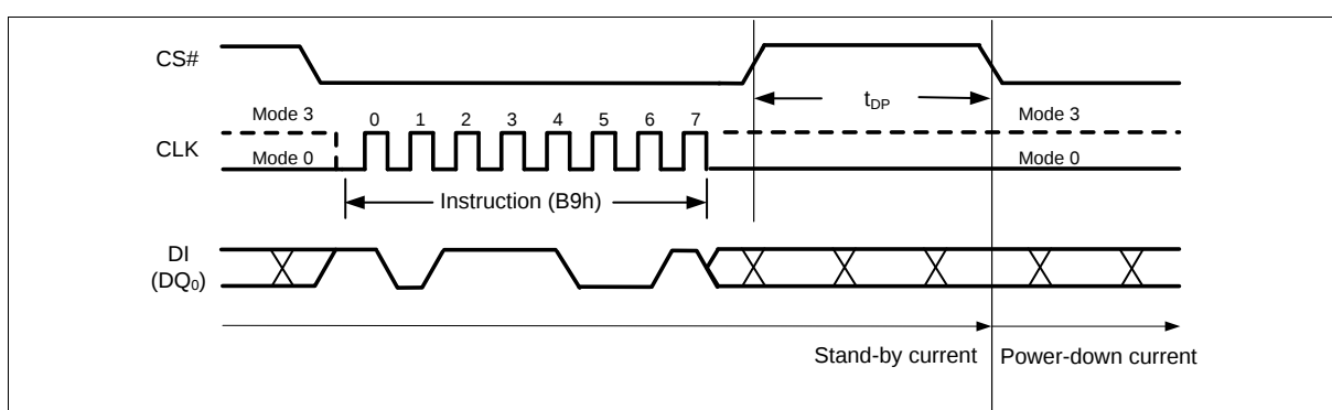
Figure 42 Deep Power-down Instruction (SPI Mode)
