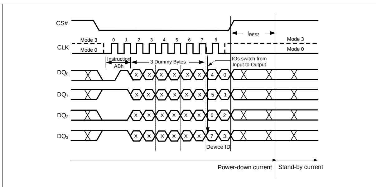
Figure 47 Release Power-down / Device ID Instruction (QPI Mode)
