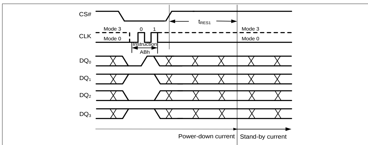
Figure 45 Release Power-down Instruction (QPI Mode)
