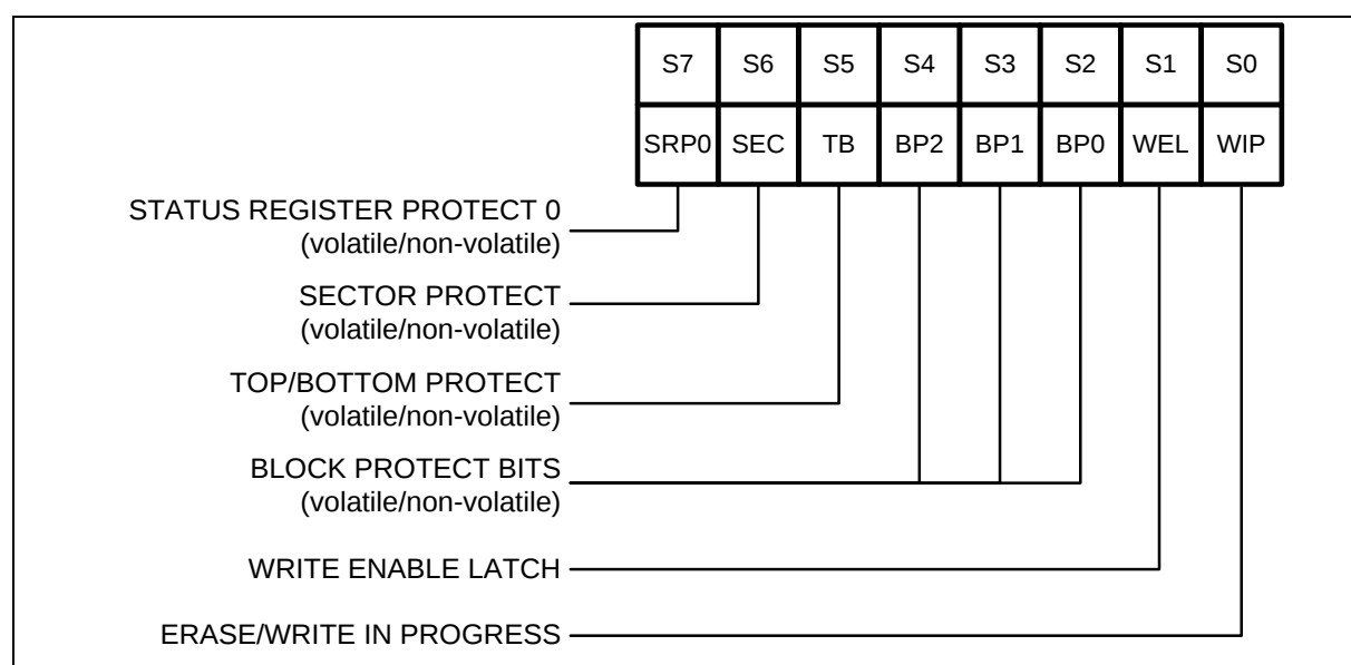
Figure 5 Status Register-1
