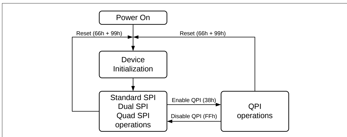
Figure 2 FM25LQ32I3 Serial Flash Memory Operation Diagram
