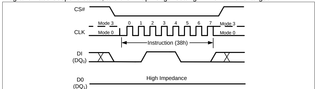
Figure 62 Enable QPI Instruction (SPI Mode only)
