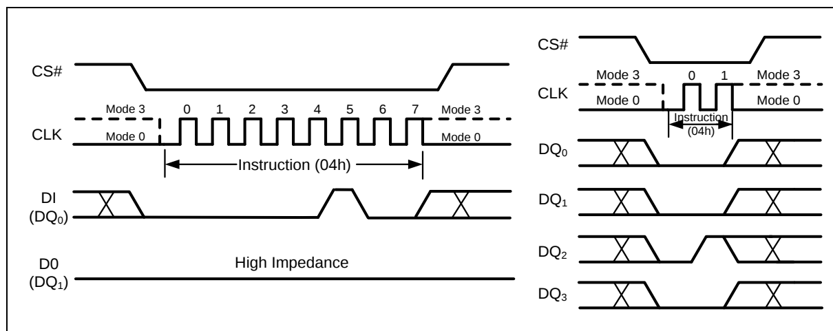
Figure 10 Write Disable Instruction for SPI Mode (left) or QPI Mode (right)
