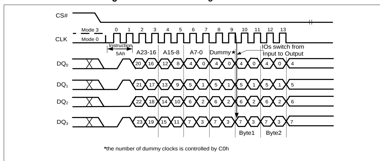
Figure 56 Read SFDP Register Instruction (QPI Mode)
