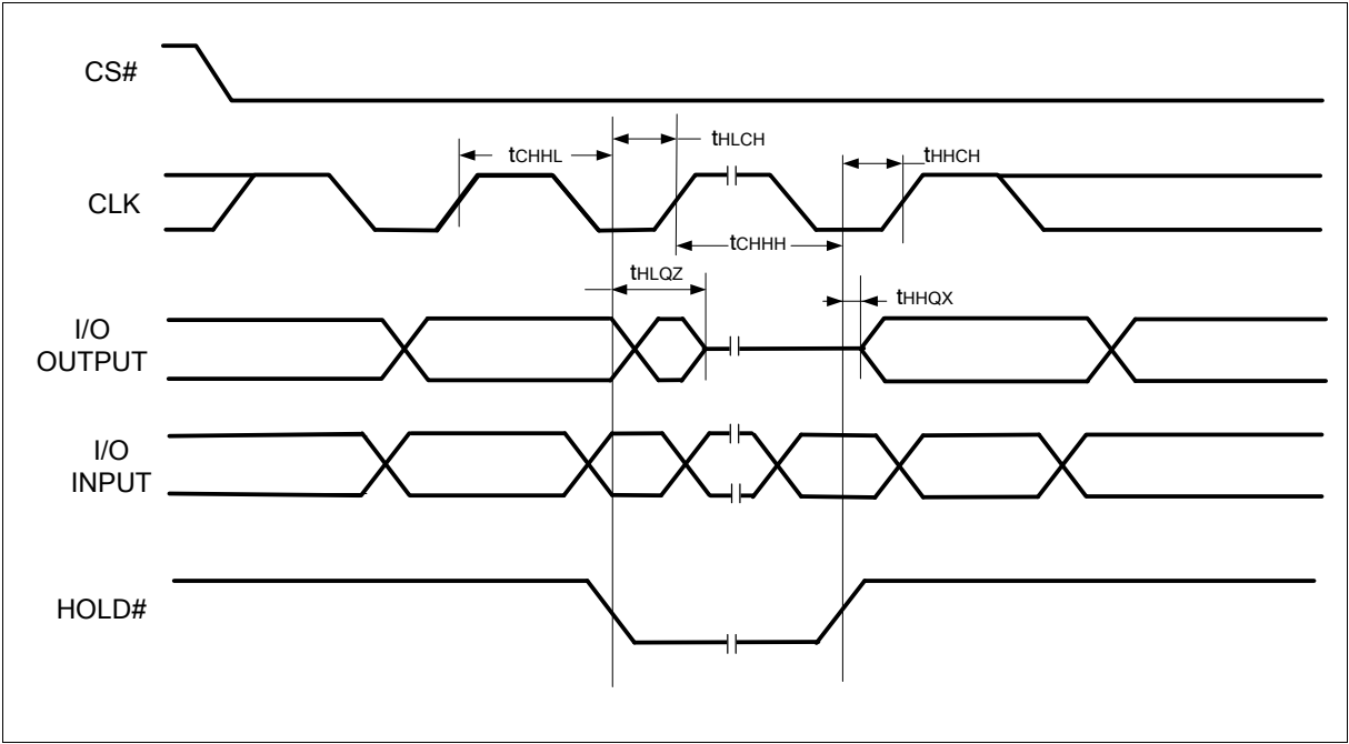
Figure 80 Hold Timing
