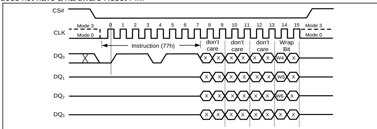
Figure 27 Set Burst with Wrap Instruction for SPI Mode
