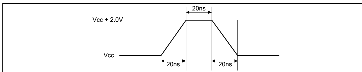
Figure 75 Maximum Positive Overshoot Waveform
