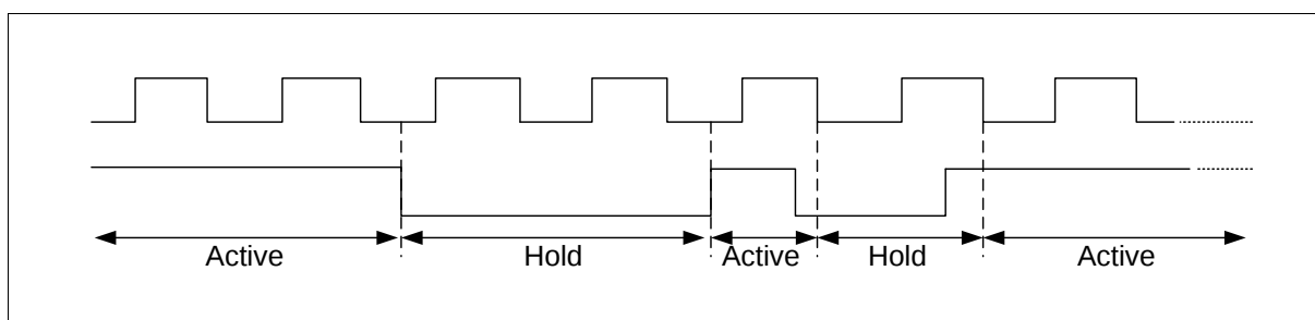
Figure 4 HoldCondition Waveform
