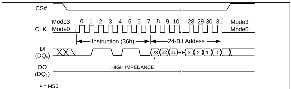
Figure 64 Individual Block/Sector Lock Instruction(SPI)
