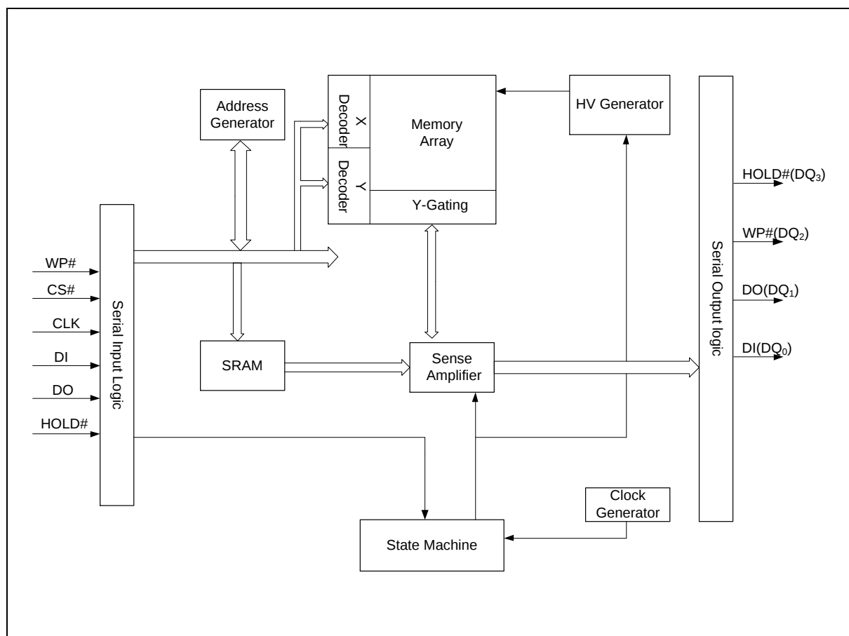
Figure 1 FM25LQ32I3 Serial Flash Memory Block Diagram
