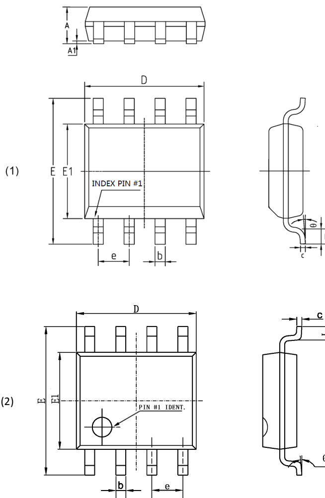
SOP8 (150mil)
