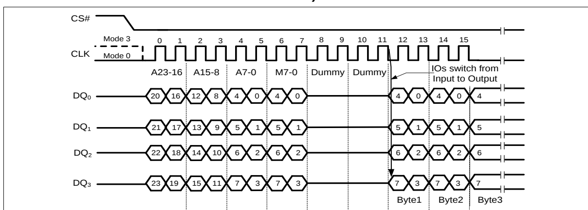
Figure 25 Fast Read Quad I/O Instruction (Previous instruction set M5-4 = 10, SPI Mode)
