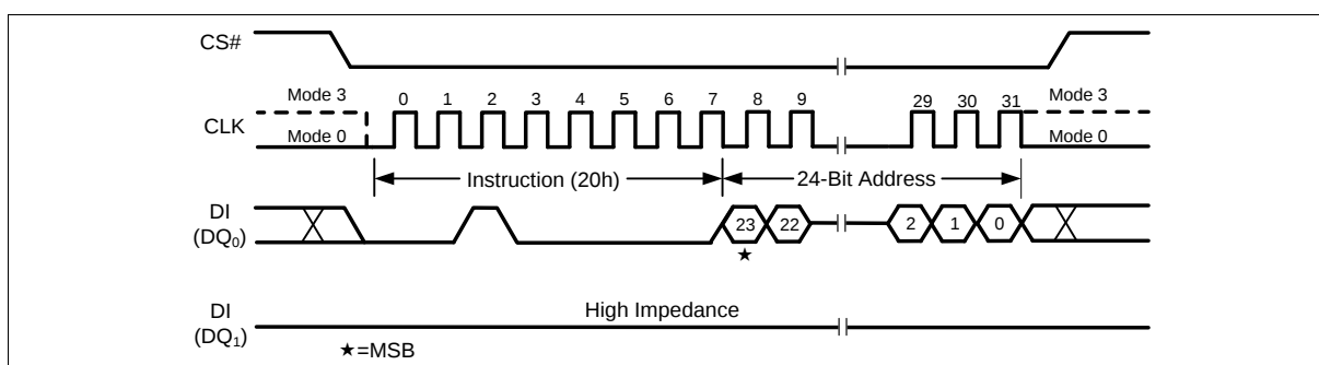
Figure 31 Sector Erase Instruction (SPI Mode)
