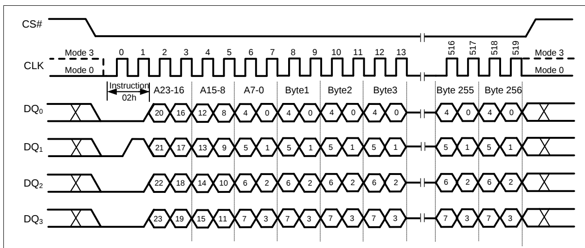
Figure 29 Page Program Instruction (QPI Mode)
