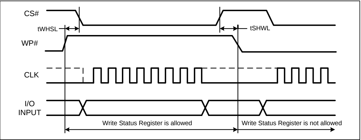
Figure 81 WP# Timing
