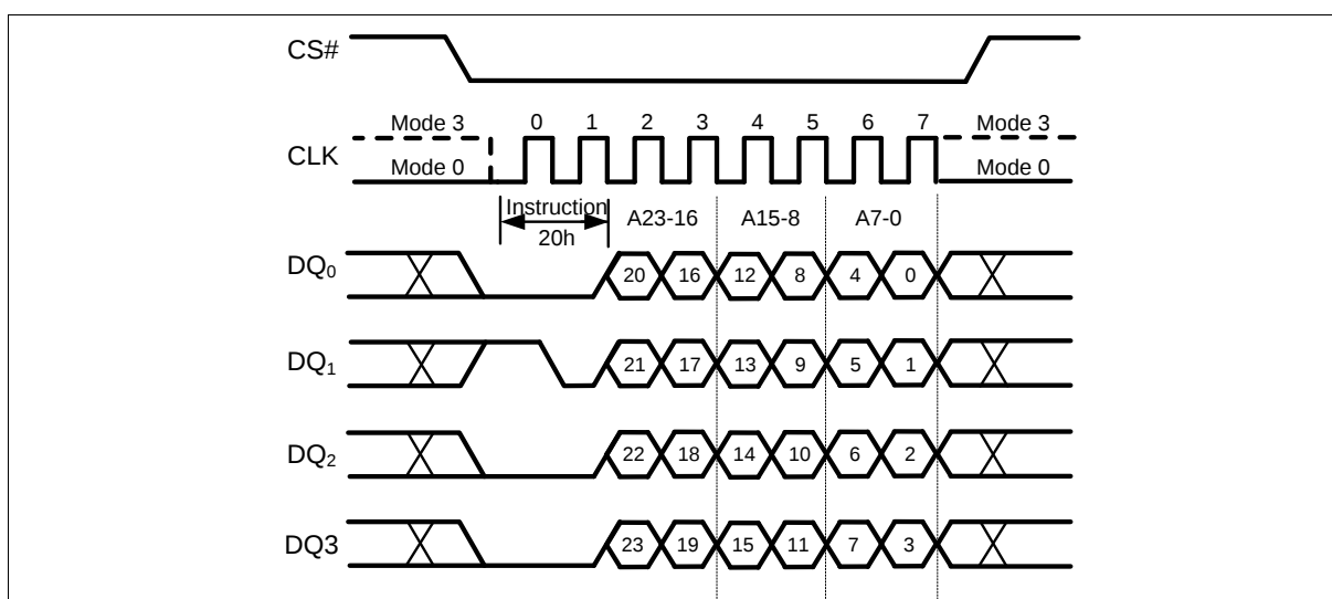
Figure 32 Sector Erase Instruction (QPI Mode)
