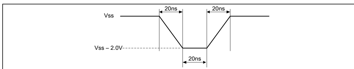
Figure 74 Maximum Negative Overshoot Waveform
